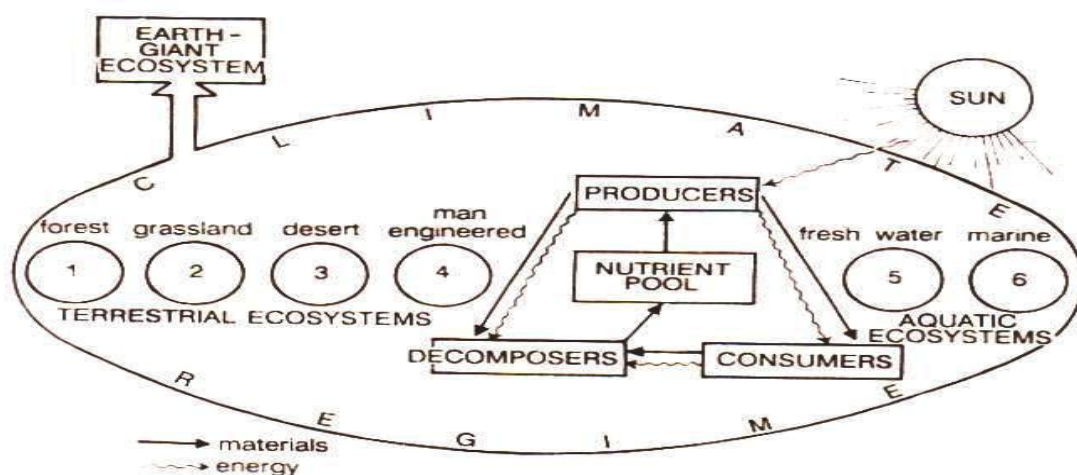
Diagrammatic representation of the basic types of ecosystems, all of which together constitute the giant ecosystem—the biosphere. Note, in the centre, the generalised scheme of the structure and function of any unit ecosystem of the biosphere.
