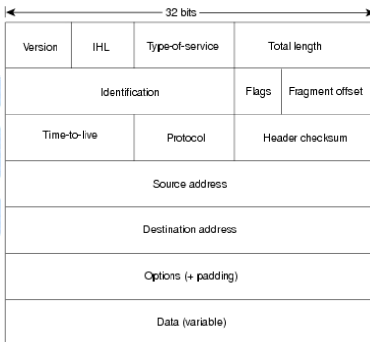
IP Packet Format
