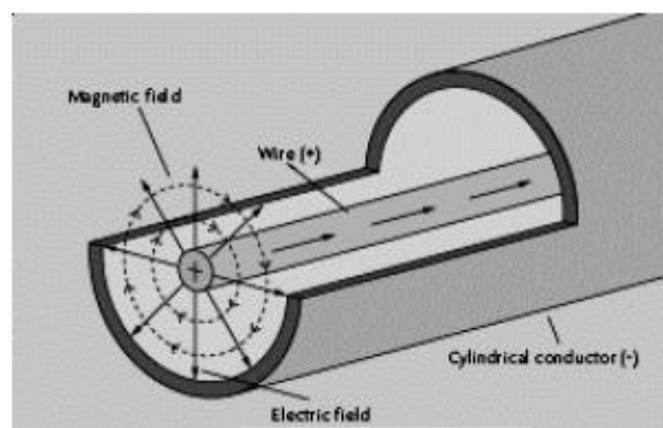
Coaxial Cable
